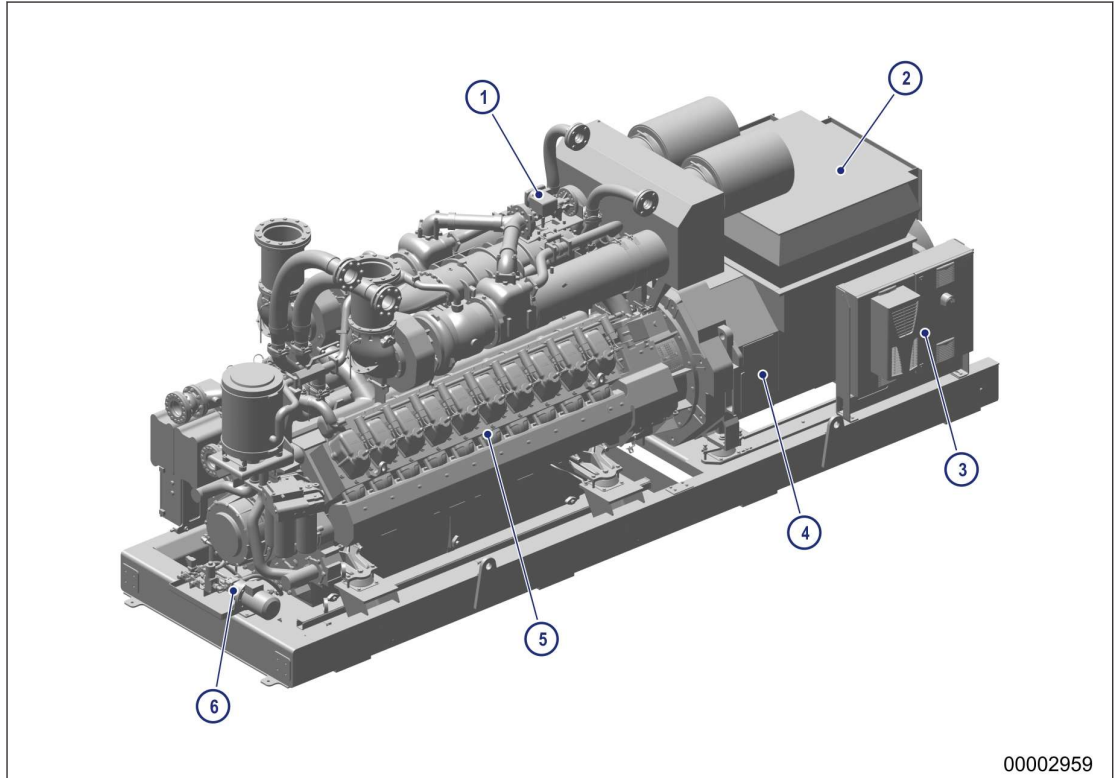
Figure 3: Engine-generator set - 20V engine, engine side
