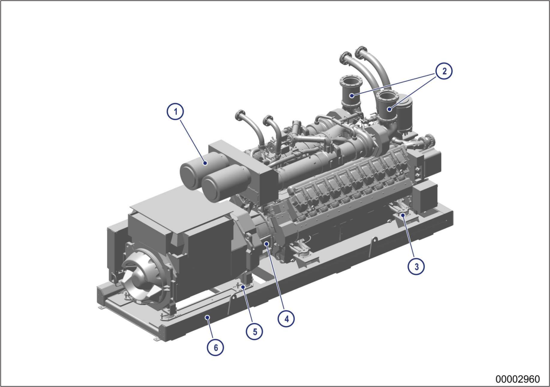
Figure 5: Engine-generator set – 20V engine, generator side
