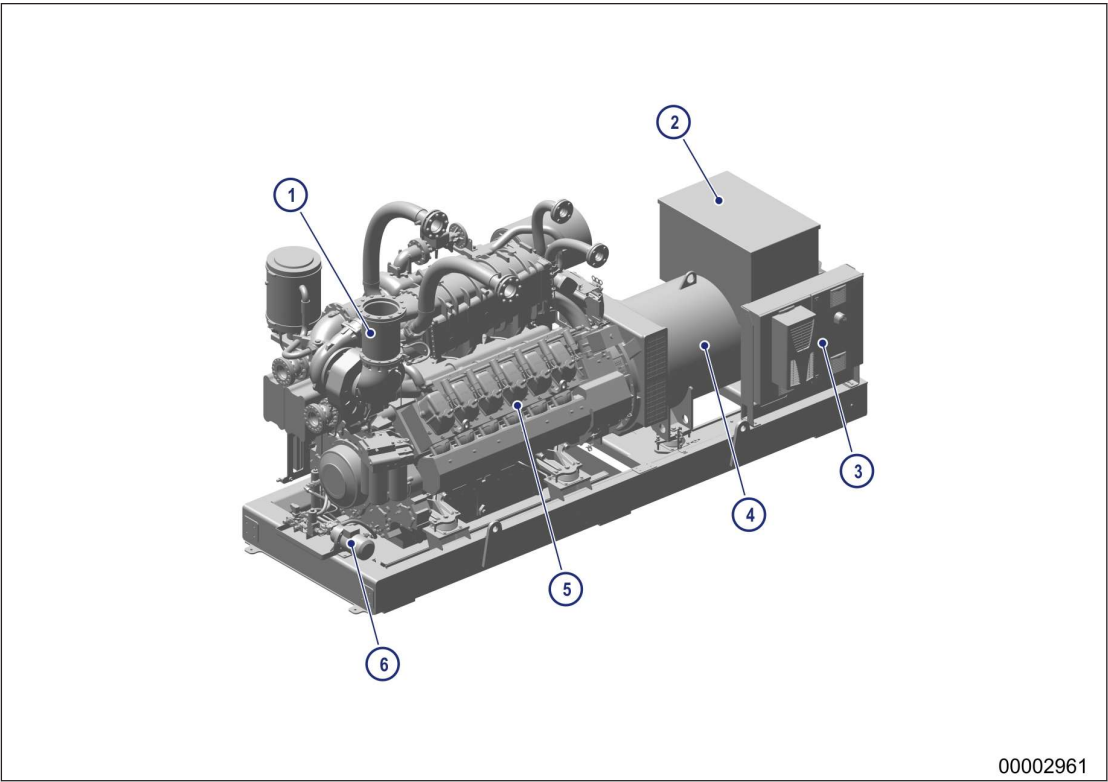
Figure 4: Engine-generator set – 12V engine, engine side
